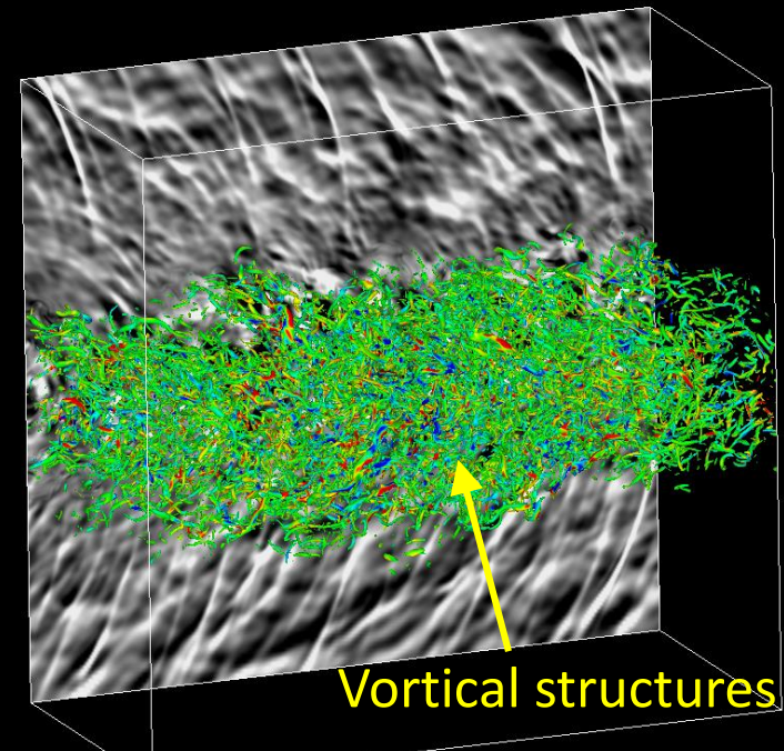
Supersonic jet and noise radiation
