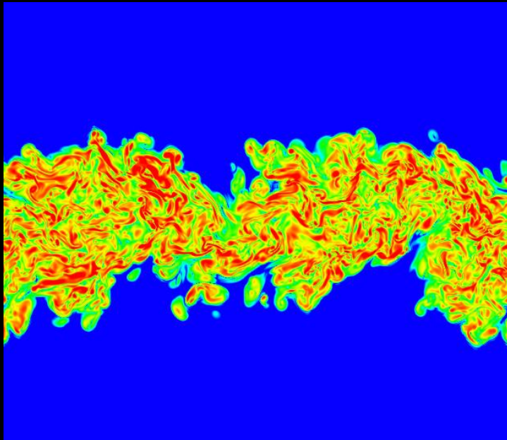
Enstrophy in supersonic jet
